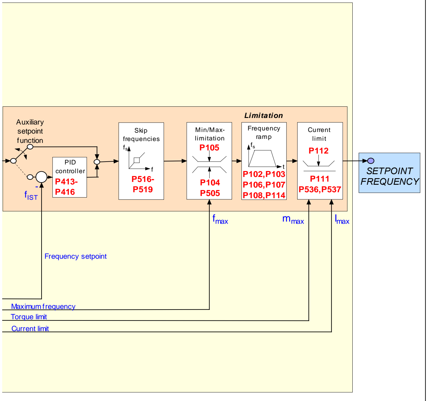
Fig. 14: Setpoint processing
